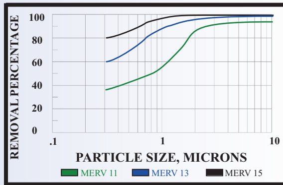
MINIMUM PARTICLE SIZE EFFICIENCY Test Filter Size 24" x 24" x 4" Nominal
